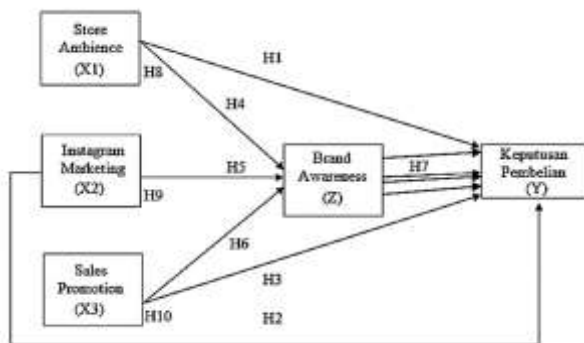
Gambar 3. Hipotesis Penelitian
